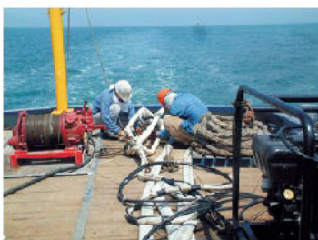
MASW-equipment (air gun and hydrophone string)
