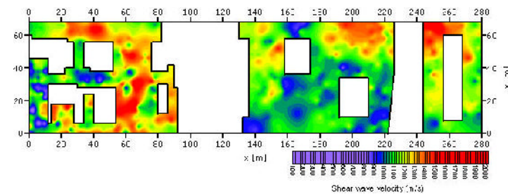
Plan view of s-wave velocity of a bridge construction site. The survey was carried out when cavities were found.
